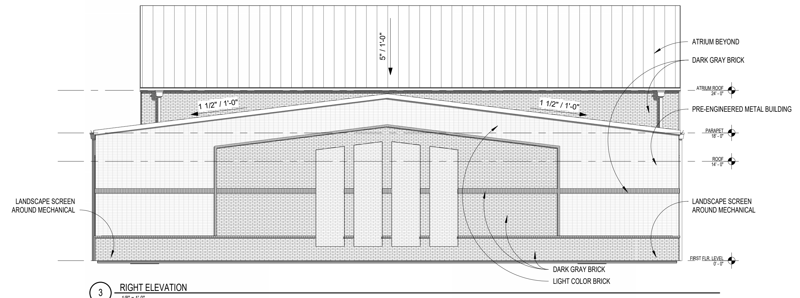
3 RIGHT ELEVATION 1/8" = 1'-0"
