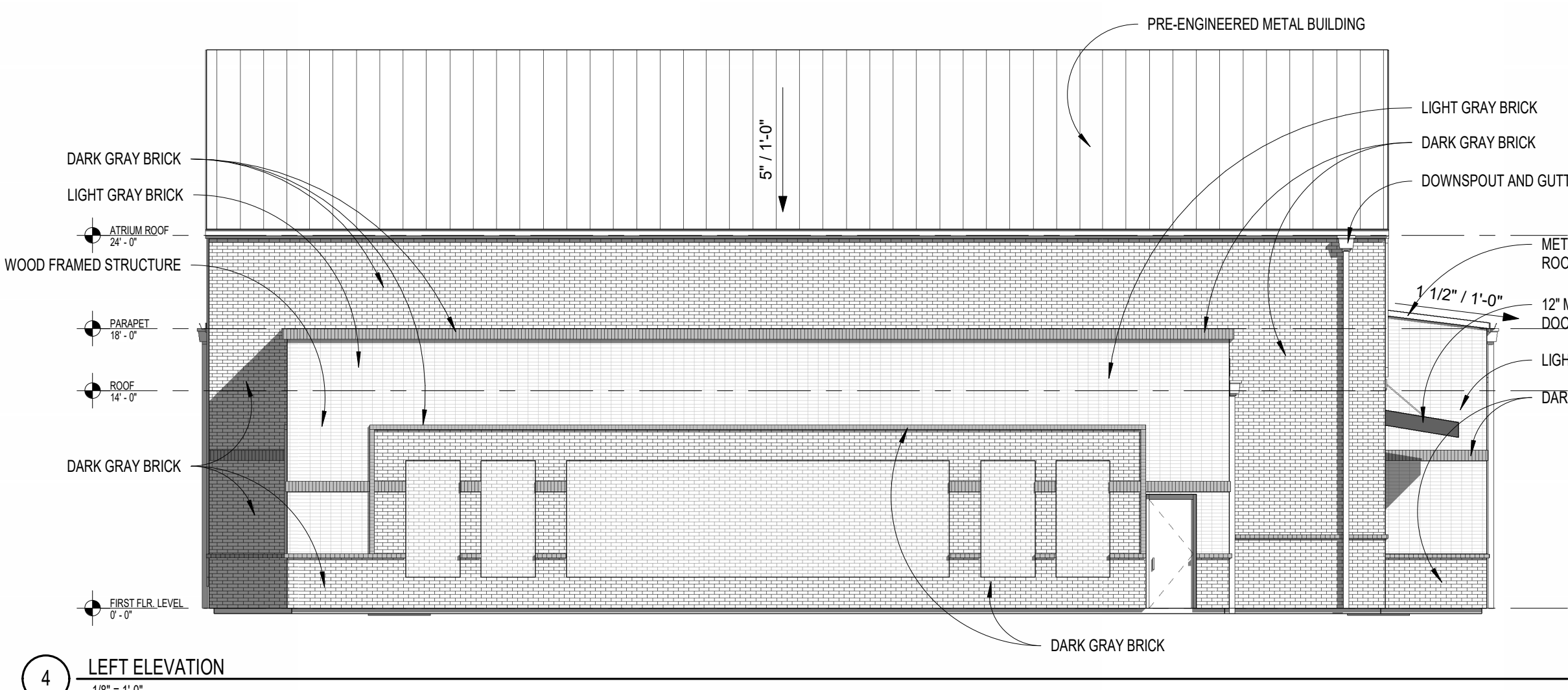
4 LEFT ELEVATION 1/8" = 1'-0"
